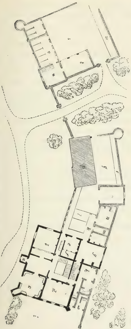
[Fig. 176. Ground plan of house and offices in the castle-gothic.]
